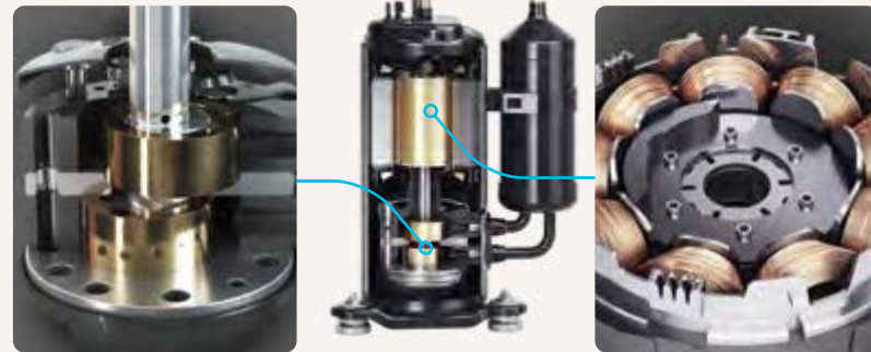
Twin Rotary Compressor
